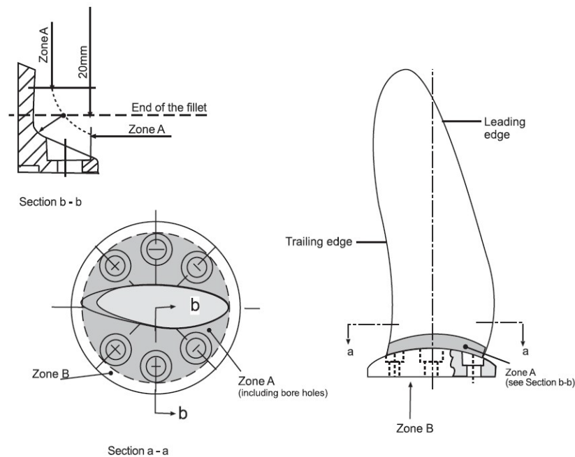
Fig. 1.2.2-3 Severity zones for controllably pitched and built-up propeller blade
