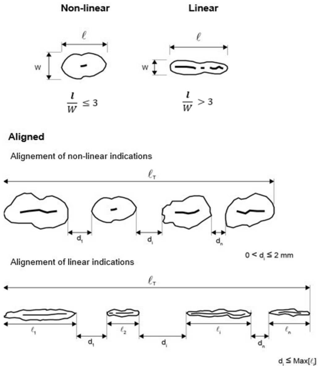
Fig. 2.3.1 Shape of indications
