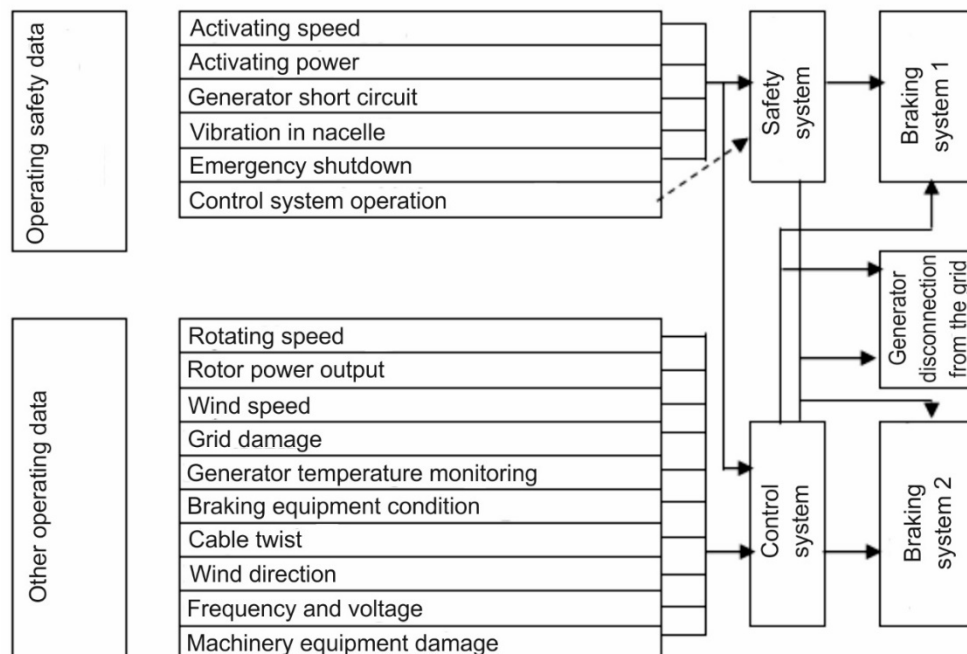
Fig. 2 – Example of interaction of control and safety systems
