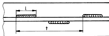
a) staggered weld
