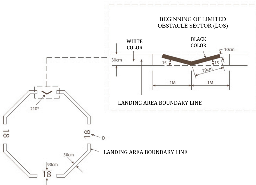
Fig. 5.6.2.4 Dimensions and arrangement of the landing area marking (example – octagonal landing area)
