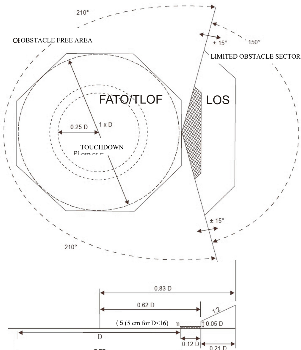
Fig. 4.1-1. Free obstacle area and limited obstacle sector (LOS). TLOF diameter 1D
