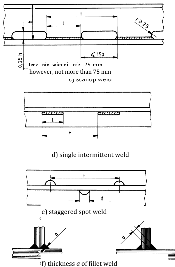
Fig. 4.1.3.1 Types of fillet welds and determination of weld thickness
