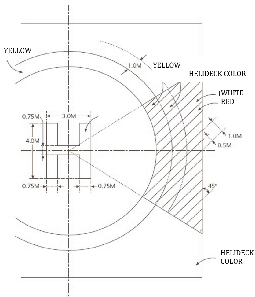
Fig. 5.6.3-1. Dimensions of the mark of prohibited touch-down direction
