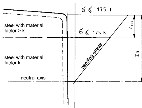
Fig. 15.6.1. Vertical extent of HS steel application
