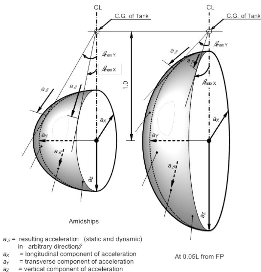
Figure 4.1 – Acceleration ellipsoid
