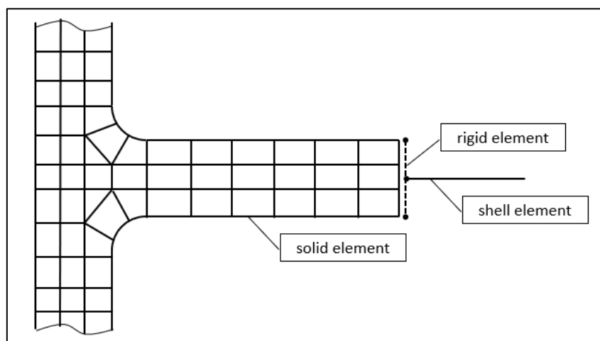
Figure 2 Transition area between solid and shell elements
