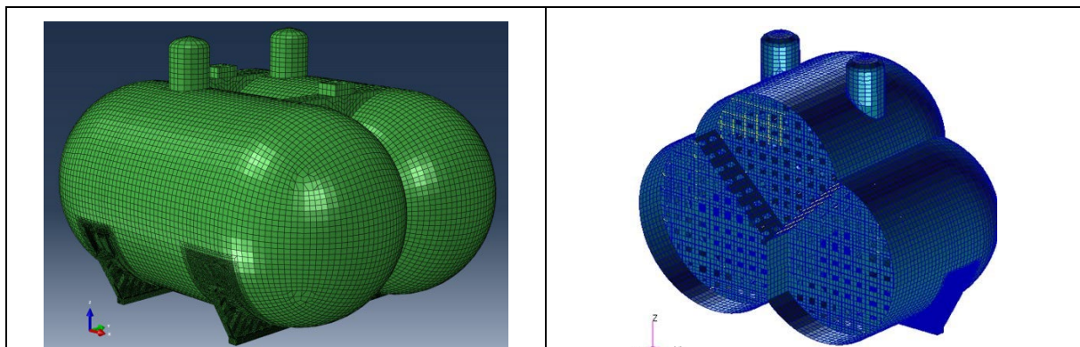
Figure 1 Finite element models of type C tanks (bi-lobe and tri-lobe)
