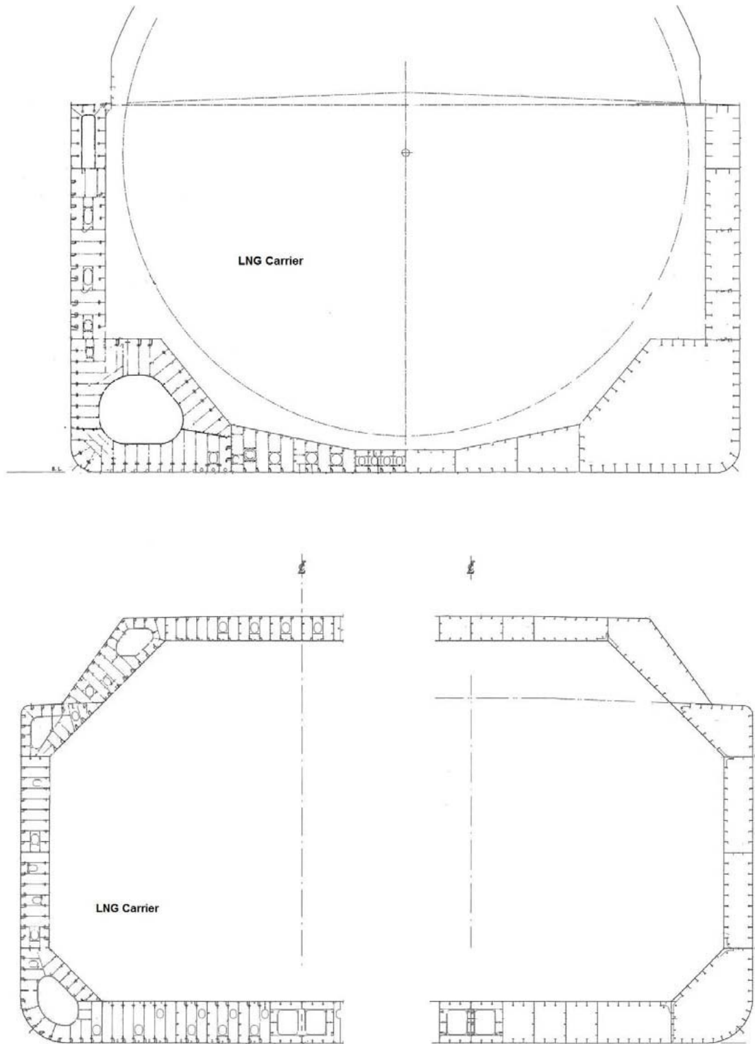
FIGURE 1 TYPICAL MIDSHIP SECTIONS OF LIQUEFIED GAS CARRIERS
