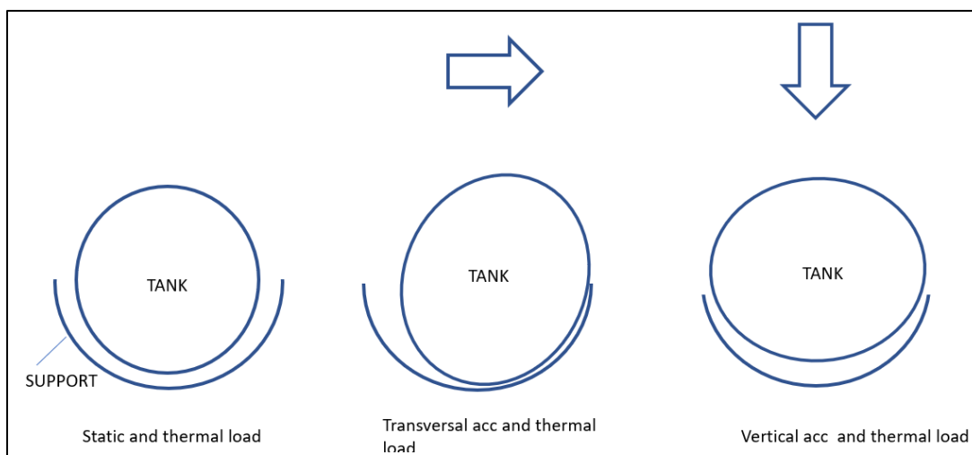
Figure 4 Contact conditions between tank and support need to allow for the relative deflection due to thermal contraction and inertial loads
