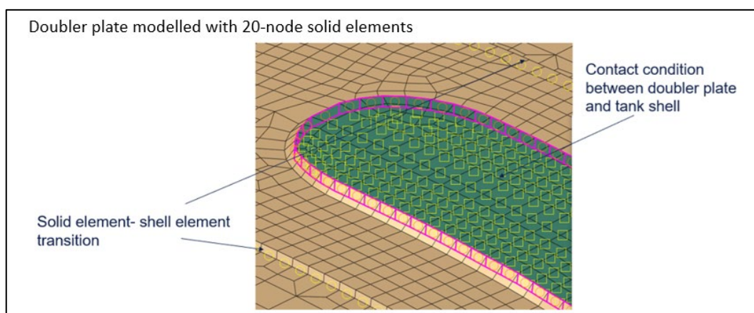
Figure 5 Recommended modelling for the doubler plate and the weld in way of tank support
