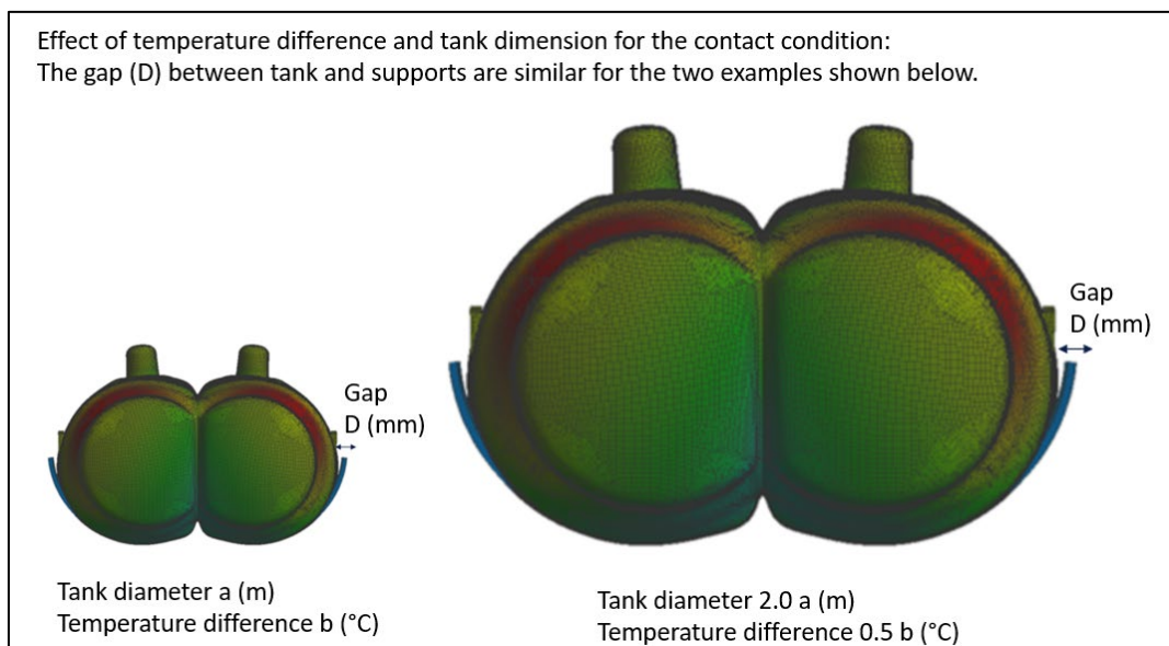
Figure 3 Modelling of contact surfaces between tank and support
