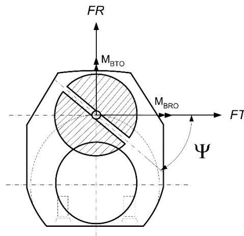
Fig. 2.1.1.2. Crankpin section through the oil bore
