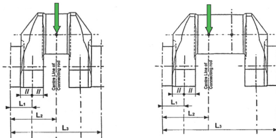
Fig. 3.4. Load applications for in-line and V-type engines
