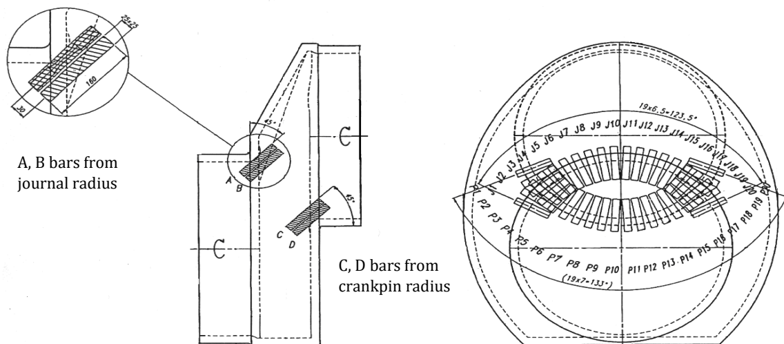
Figure 3.1. Specimen locations in a crank throw
