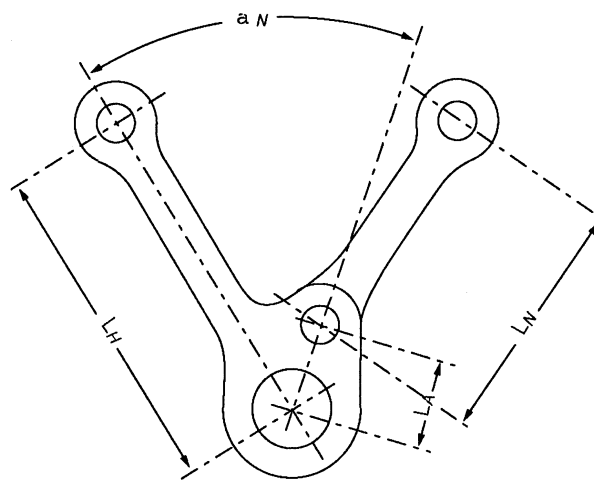
Fig. 1.3-2. Articulated-type connecting rod
