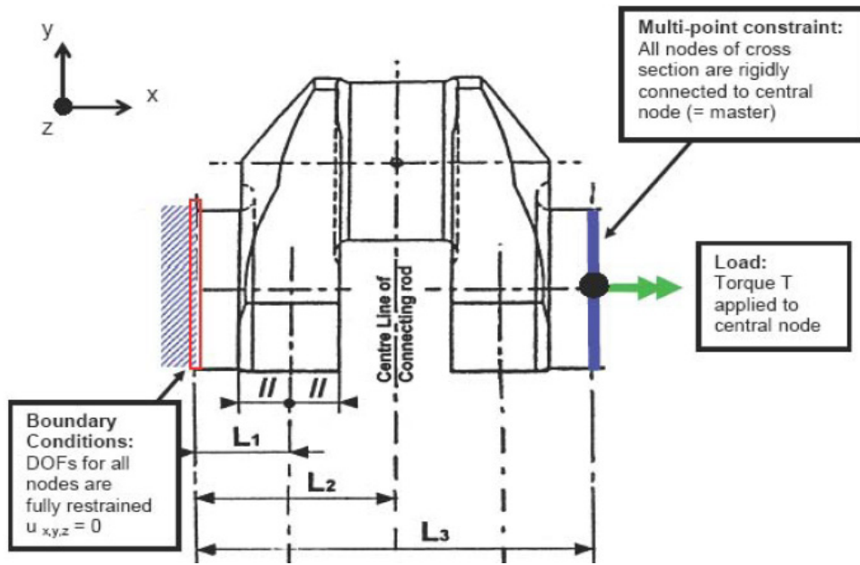
Fig. 3.1. Boundary and load conditions for the torsion load case
