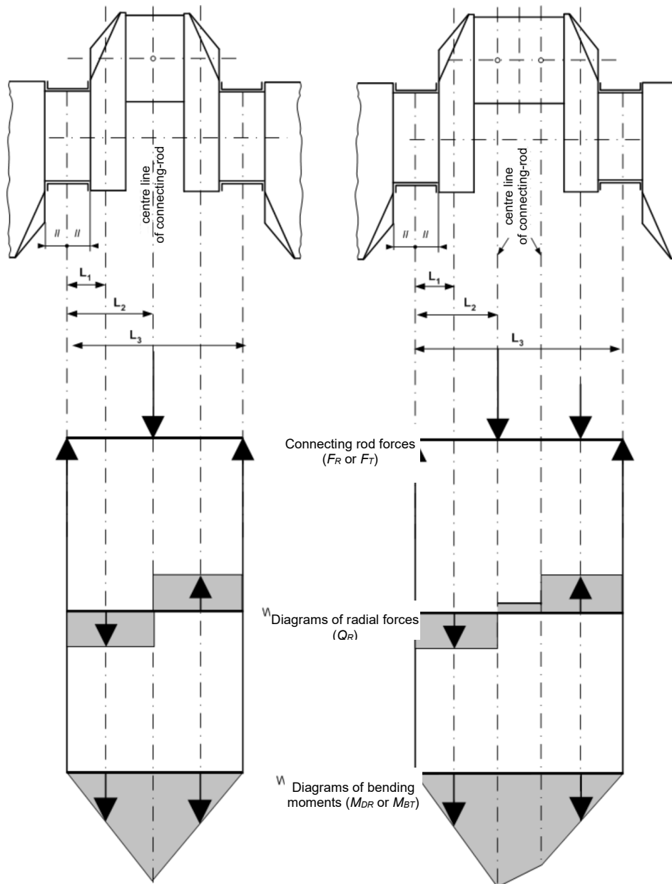
Fig. 2.1.1.1. Crank throw for in-line engine and for V-type engine with 2 adjacent connecting rods
