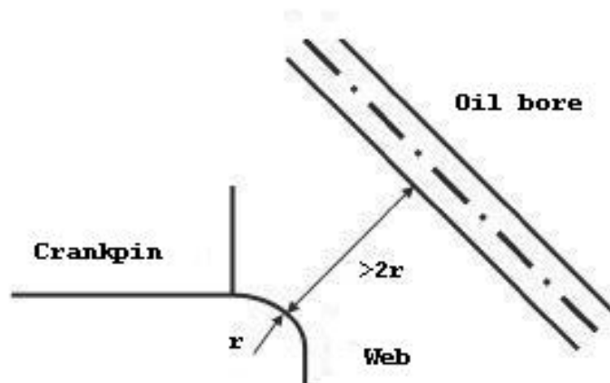
Fig. 2.1. Oil bore proximity to fillet
