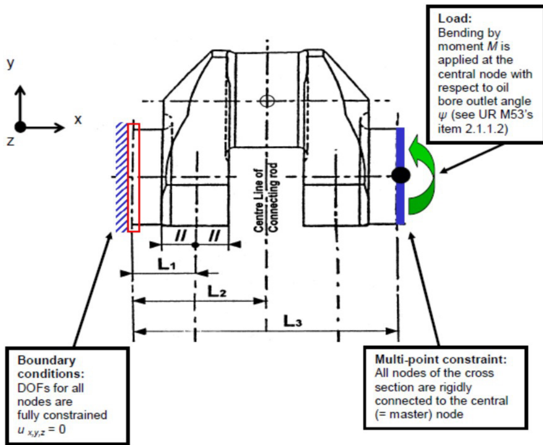
Figure 3.2. Boundary and load conditions for the pure bending load case
