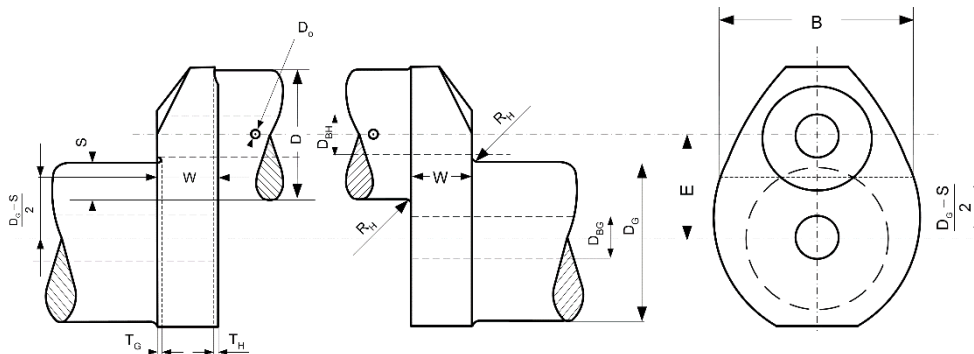
Fig 3.1. Crank dimensions necessary for the calculation of stress concentration factors
