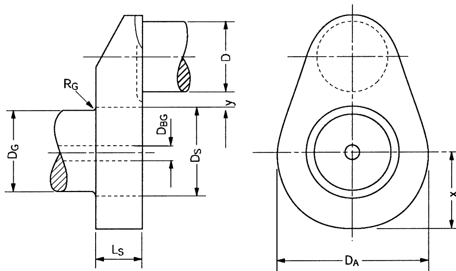
Fig. 7.1. Crank throw of semi-built crankshaft
