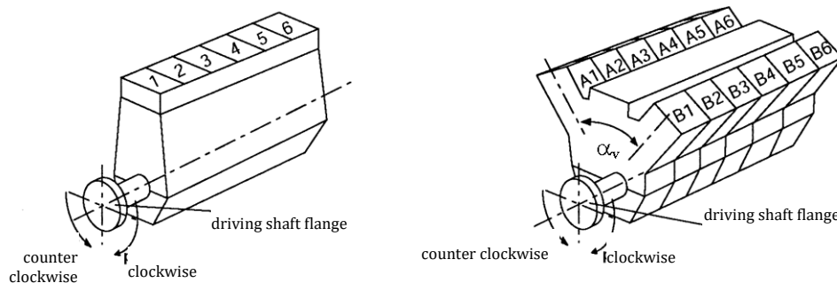
Fig. 1.3-1. Cylinders configuration
