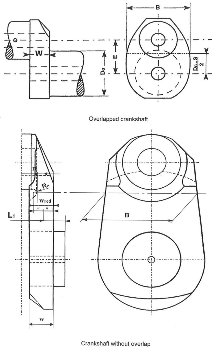
Fig. 2.1.1.1. Reference area of crank web cross-section
