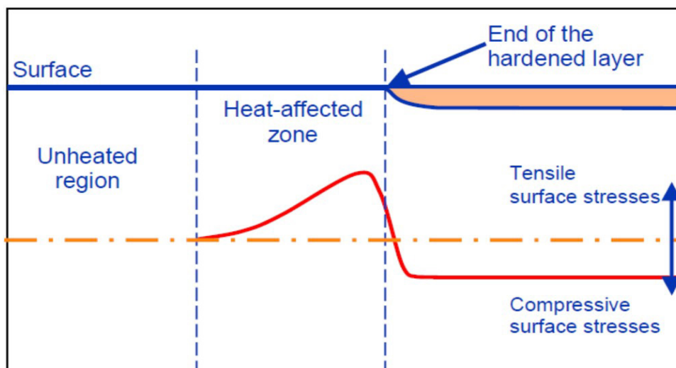
Figure 4.2. Residual stresses along the surface of a pin and fillet
