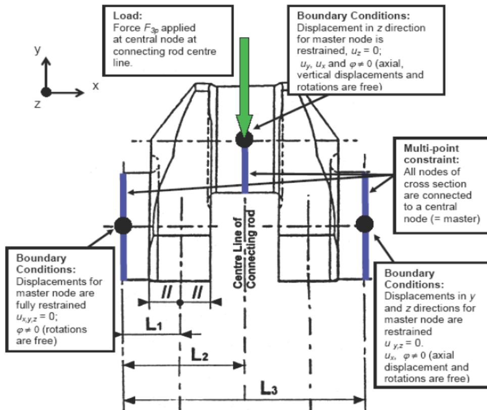
Fig. 3.3. Boundary and load conditions for the 3-point bending load case of an in-line engine
