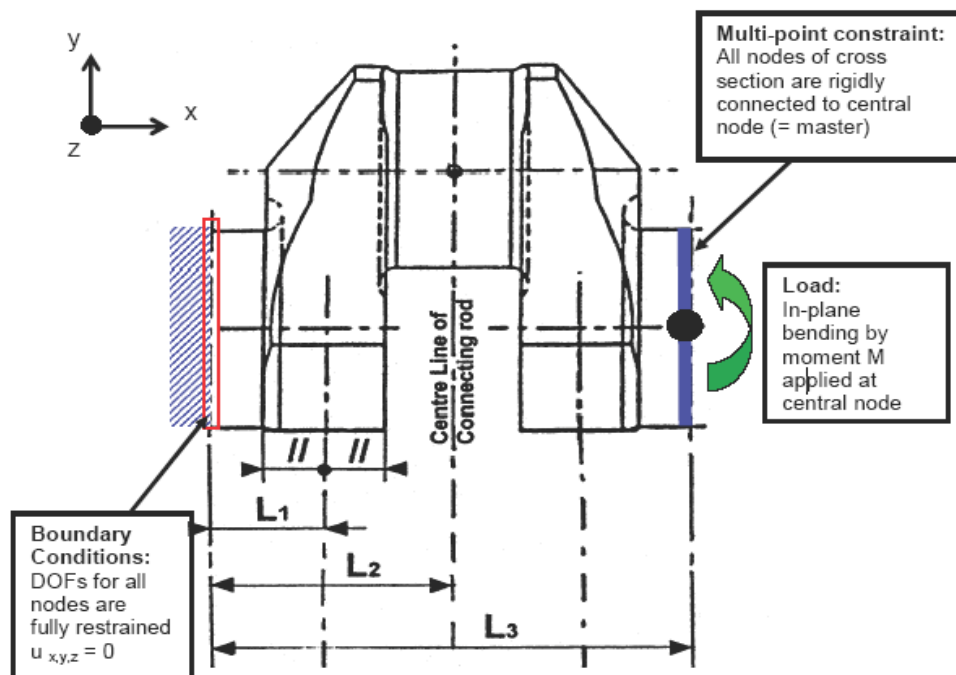
Fig. 3.2. Boundary and load conditions for the pure bending load case
