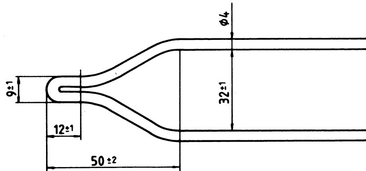
Fig. 2.25.3-1. Filament loop (dimensions in mm).
