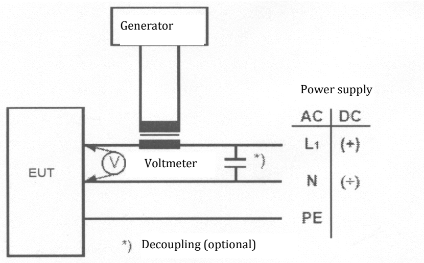
Fig. 2.19. Test set-up – conducted low frequency test
