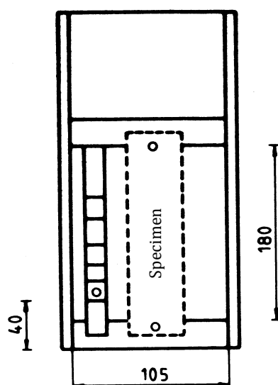
Fig. 2.25.3-3. Grip for specimen with scale (dimensions in mm).
