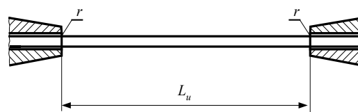
Fig. 22.3.2-1. The effective length L_u for wedge grips testing machine, applicable to ropes with reference number < 20 r – limiting marks for standard test, L_u – the effective length measured under zero tension
