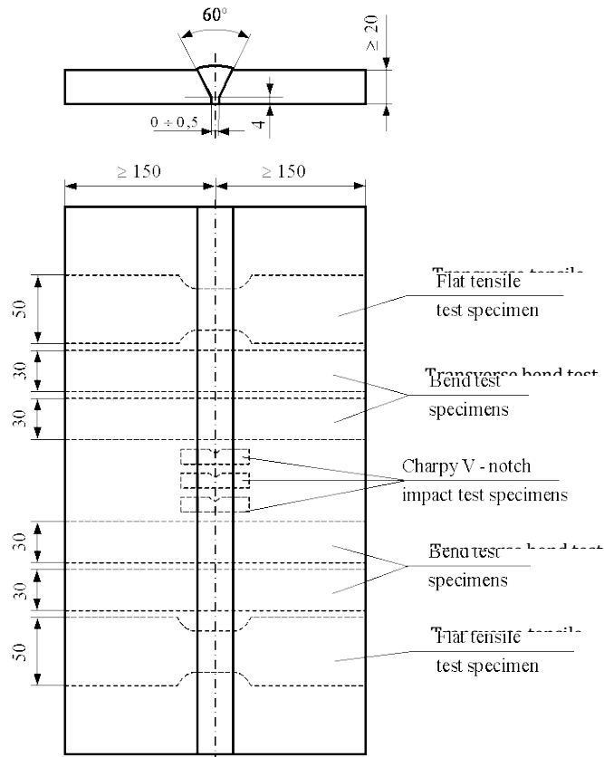
Fig. 24.6.2. Butt weld test assembly welded with multi-run technique
