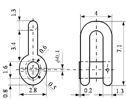
Fig. 20.3.1.1-5. Joining shackle
