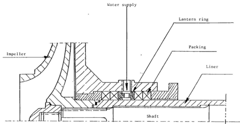
Figure 5 – Water flushed seal in chemical pump (Paragraph 15.2.7)
