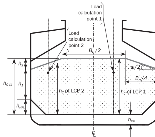
Figure 4 : Definition of the effective upper surface of cargo for a partially filled cargo hold when h_1 \geq 0
