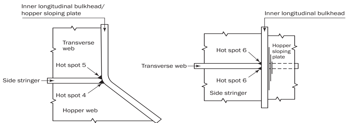
Hopper web outboard removed
