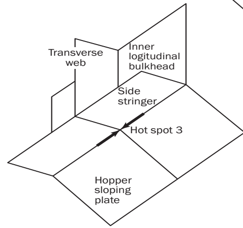
Hopper web outboard removed
