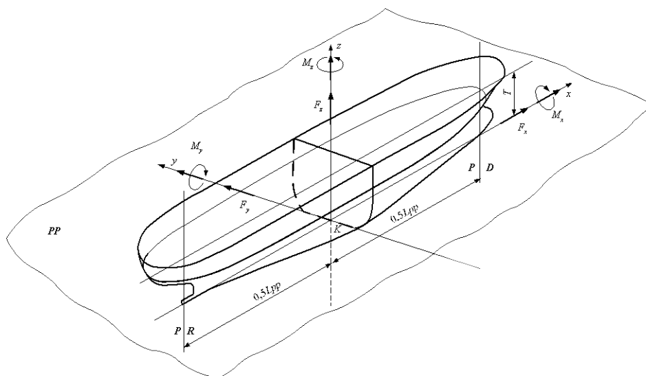
Fig. 1.2 Vessel's co-ordinate system
