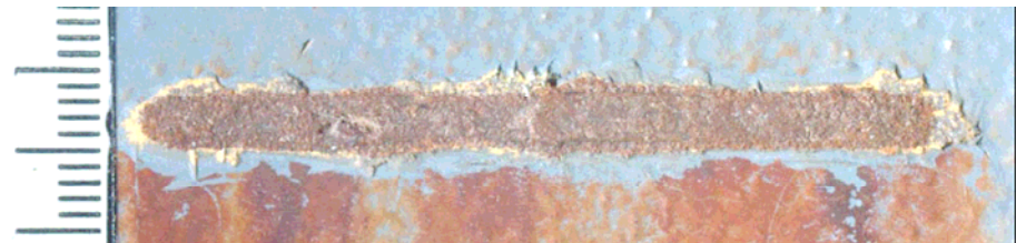
Figure C-5 Undercutting from scribe, side wave tank panel without cooling (example picture not connected with example results in this model report).
