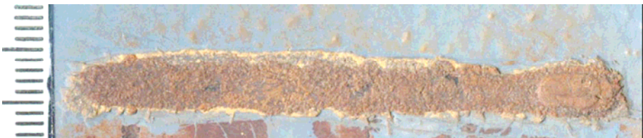
Figure C-6 Undercutting from scribe, side wave tank panel with cooling (example picture not connected with example results in this model report).
