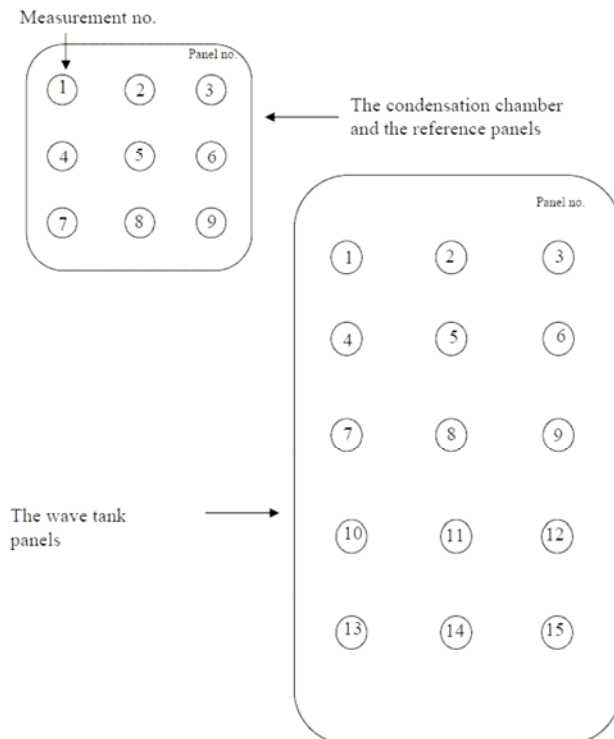
Figure B-2 Thickness measurement locations
