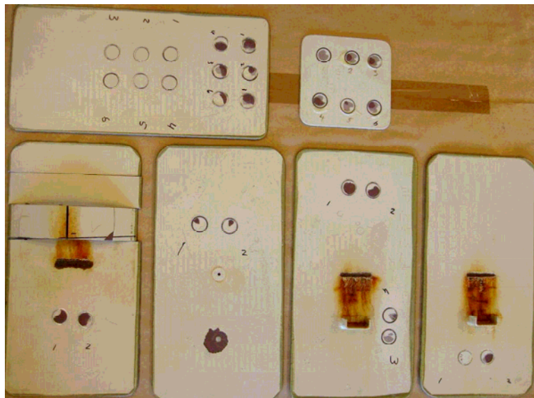
Figure C-1 Overview picture of the panels after exposure in the wave tank and the heating chamber. Reference panel not exposed – top right. Picture taken after examination (example picture not connected with example results in this model report).
