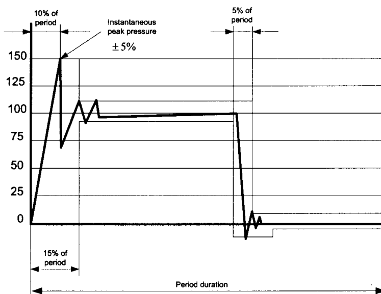
Fig 2.3.1. Impulse pressure diagram
