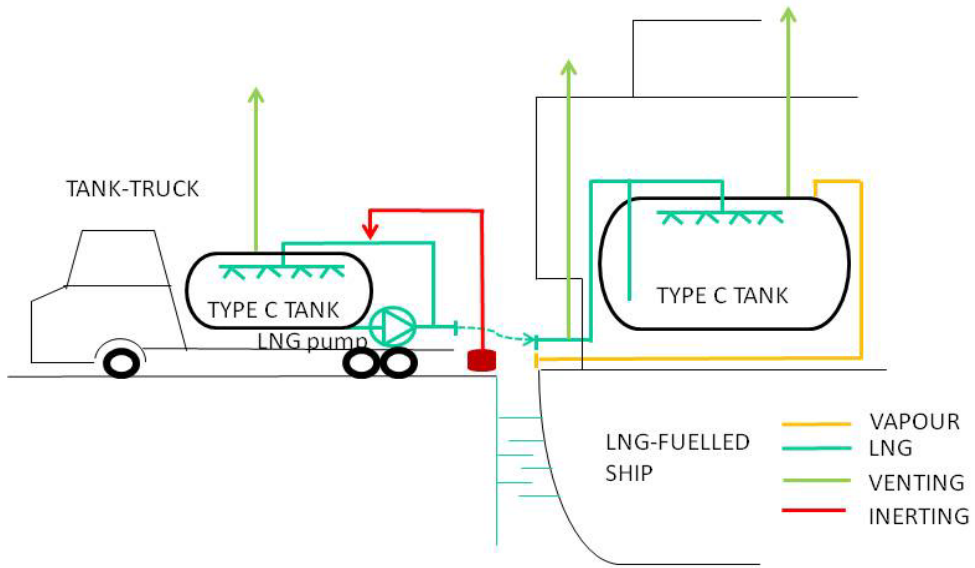
Figure 6: Truck to ship bunkering – typical arrangement of LNG fuelled ship with type C tank
