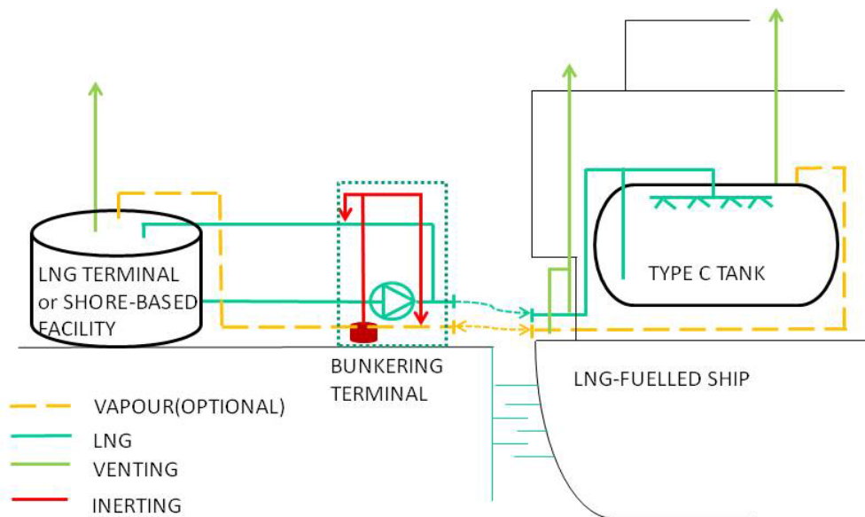
Figure 7: Terminal to ship bunkering – typical arrangement of LNG fuelled ship with type C tank
