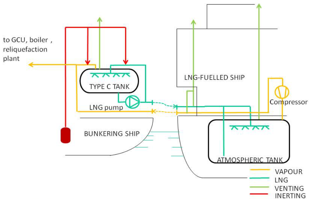
Figure 4: Ship to ship bunkering – typical arrangement of bunkering ship with type C tank and LNG fuelled ship with atmospheric tank
