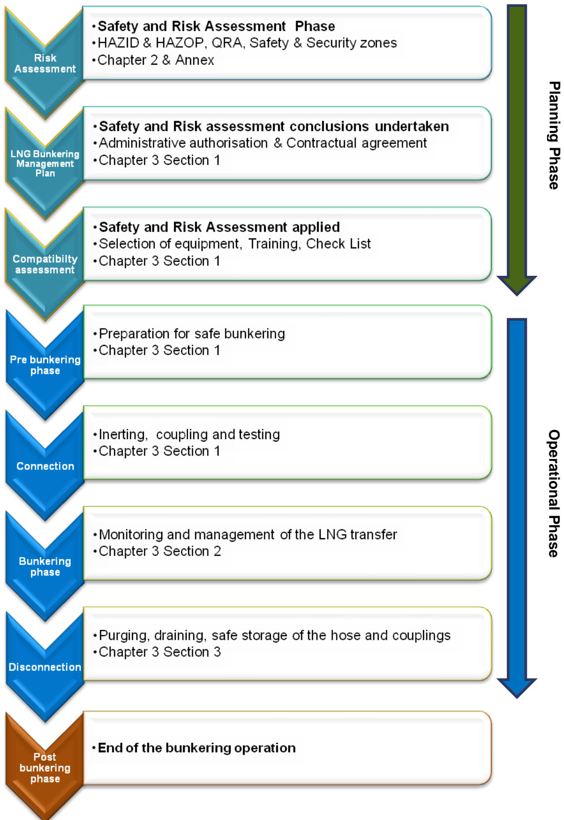
Figure 1: Bunkering process
