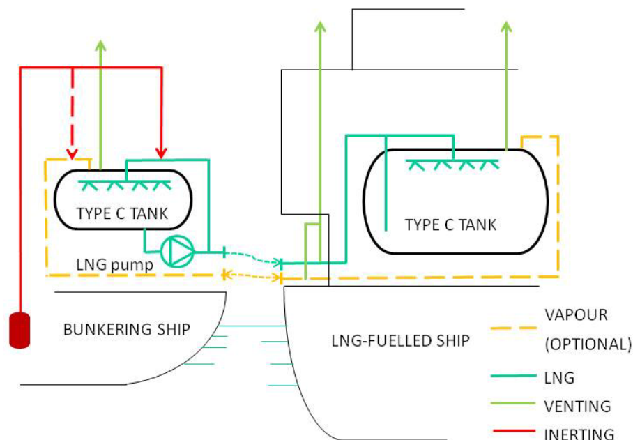
Figure 3: Ship to ship bunkering – typical arrangement of bunkering ship and LNG fuelled ship with type C tank
