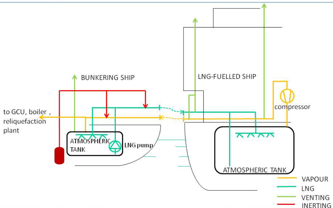
Figure 5: Ship to ship bunkering – typical arrangement of bunkering ship and LNG fuelled ship with atmospheric tank
