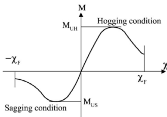
Fig. 5.3.2 Bending moment M versus curvature \chi
