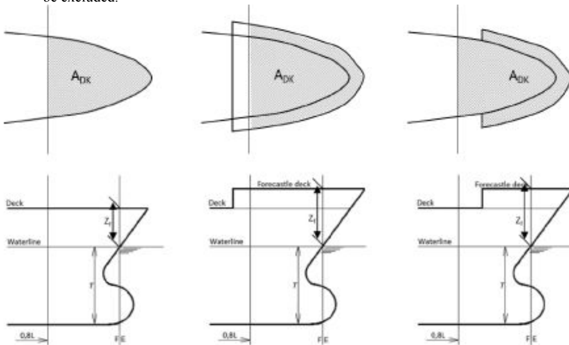
Fig. 2.3.2-1 Projected area A_{DK} and vertical distance z_f
