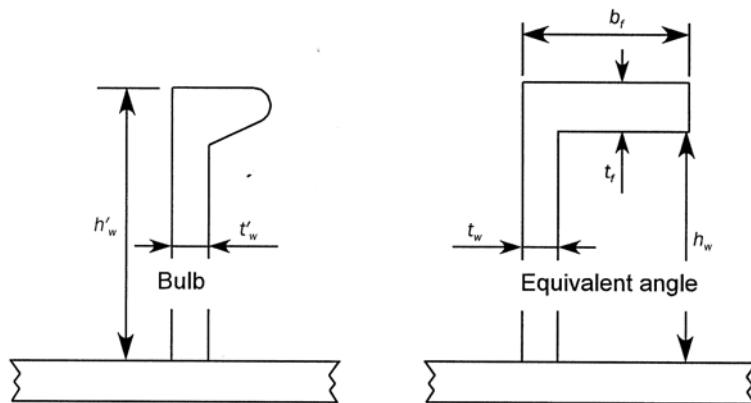
Fig. 4.3.8 Idealisation of bulb stiffener
