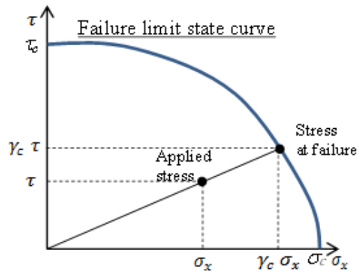
Fig. 4.3 Example of failure limit state curve and stress multiplication factor at failure
