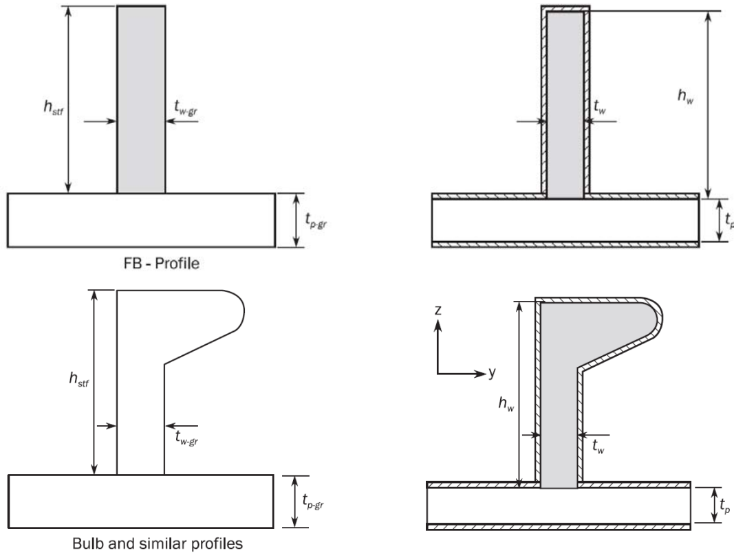
Fig. 1.3.3 Net sectional properties of supporting members
