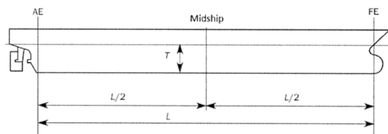
Fig. 1.2.2 Ends of length L
