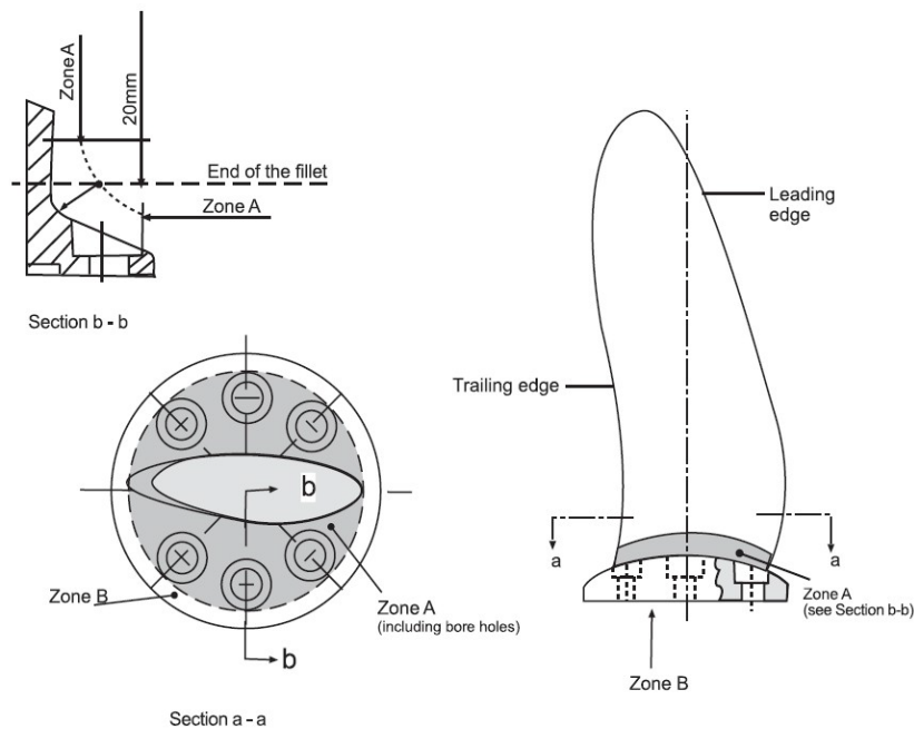
Fig. 1.2.2-3 Severity zones for controllible pitch and built-up propeller blade
