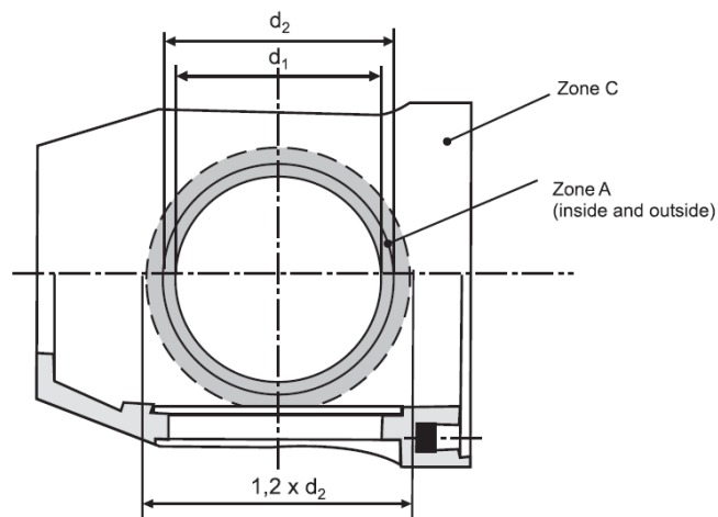
Fig. 1.2.2-2 Severity zones for controllably pitch propeller boss
