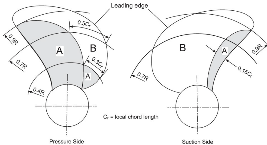
Fig. 1.2.2-1 Severity zones in blades with skew angles greater than 25^\circ
